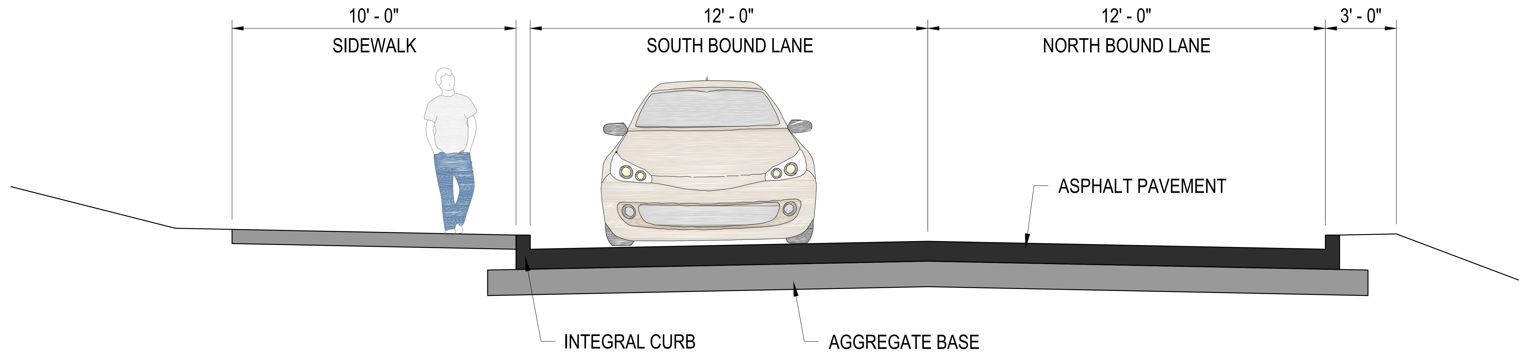
ROADWAY SECTION
