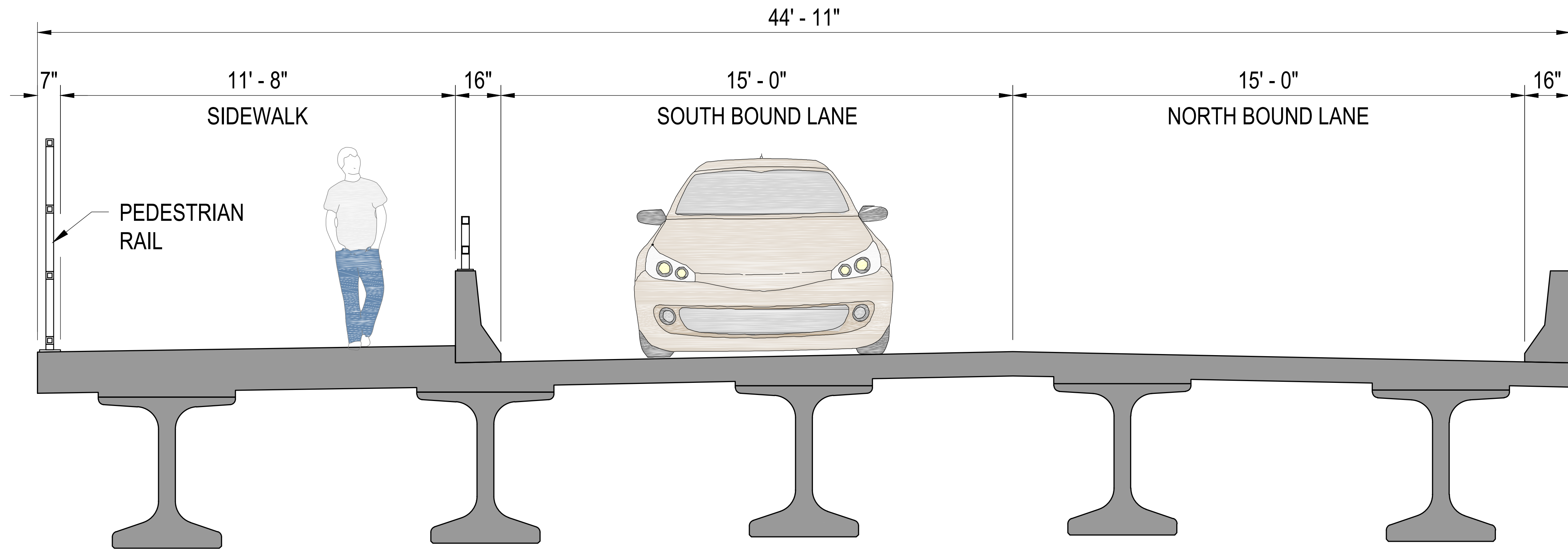
BRIDGE SECTION
